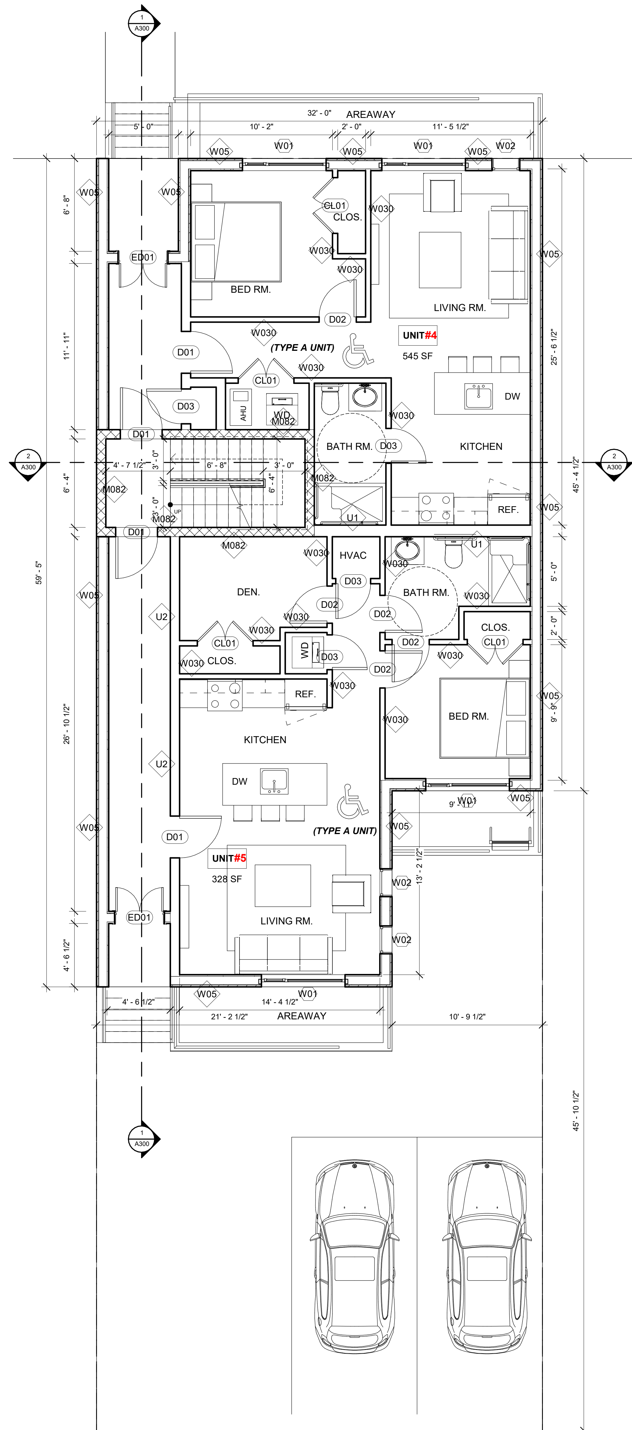
3 1ST FLOOR PLAN 1/4" = 1'-0"
